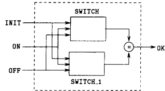
Fig. 6. Assumption-dependent equivalence of programs.
