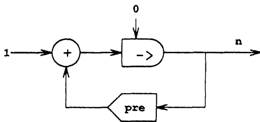
Fig. 2. Counter network.
