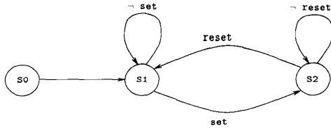
Fig. 4. The watchdog control automaton.
