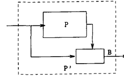
Fig. 5. Verification program.
